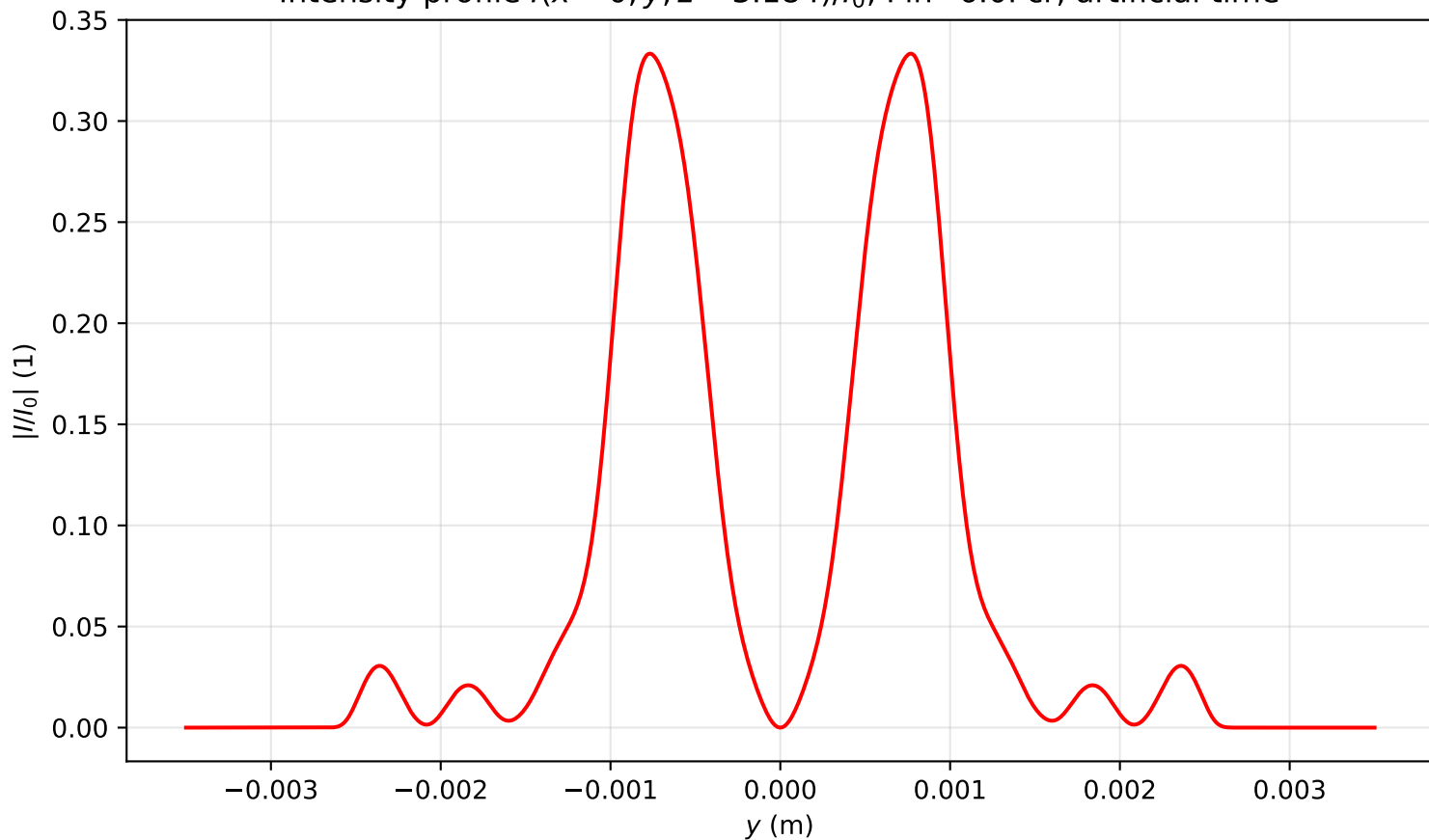
Intensity profile I(x=0, y, z=3.184)/I_0 , P_{in}=6.0P_{cr} , artificial time
